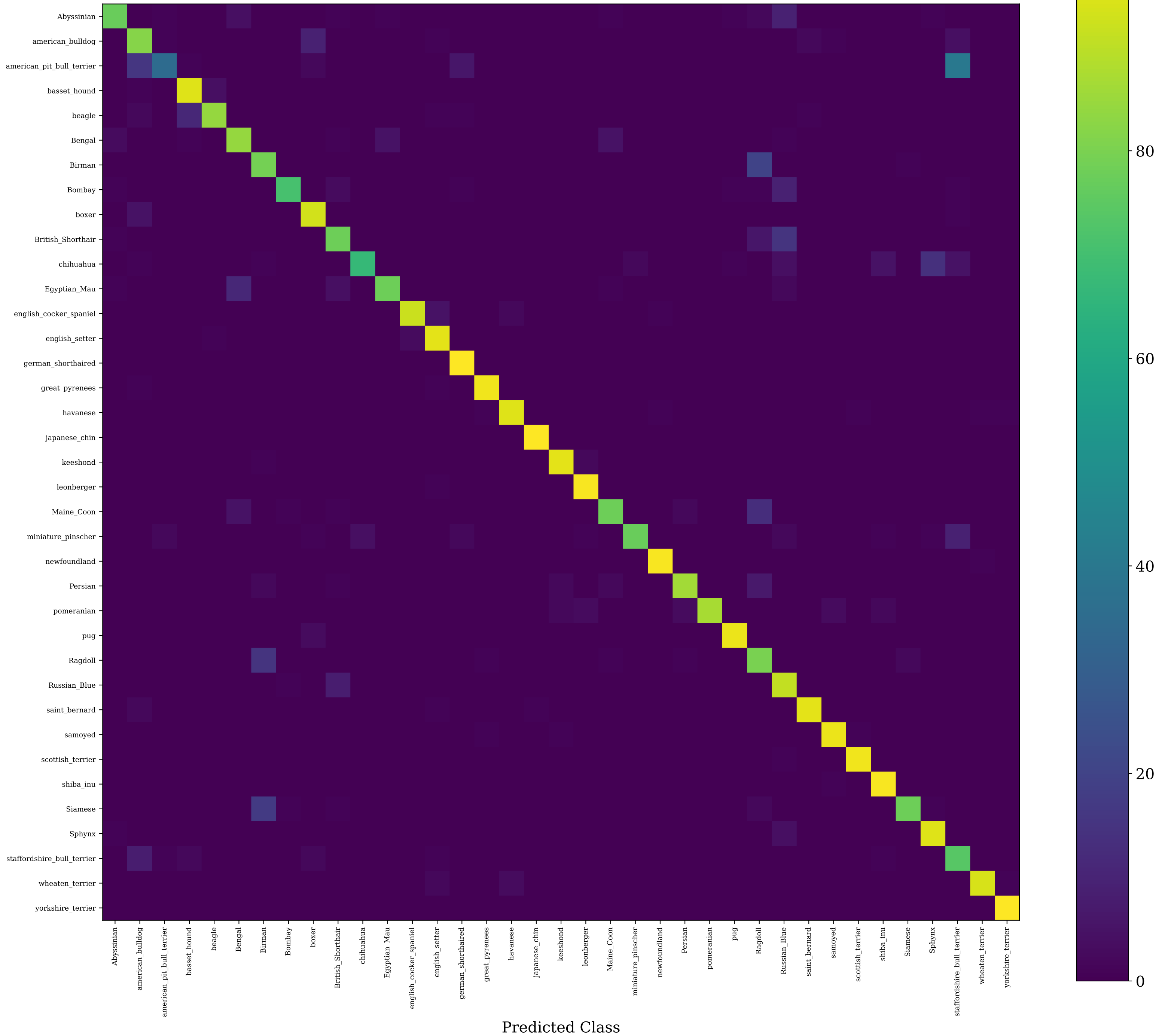
Confusion Matrix - Oxford-IIIT Pet Dataset
